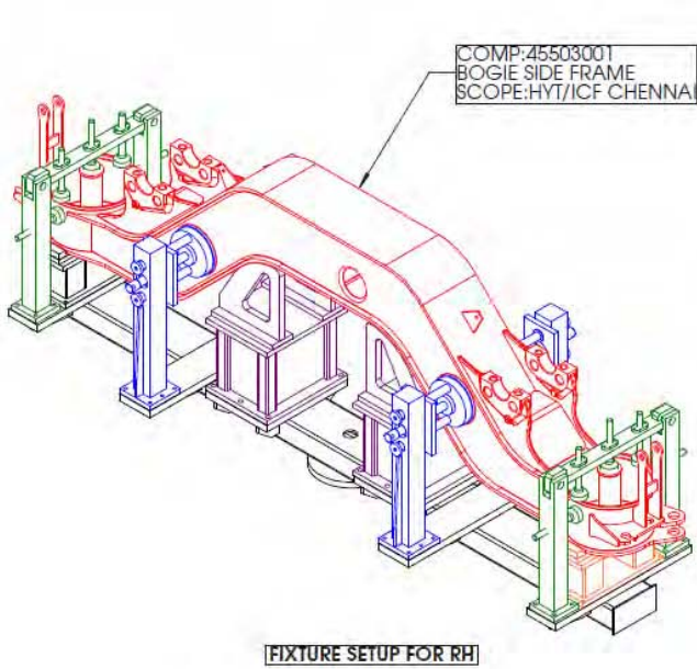
Side Frame Full Welding Fixture
