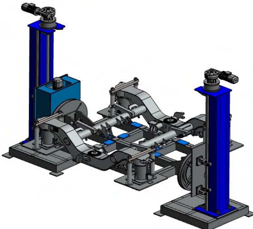
5 Ton 2 Axis Manipulator for Bogie Frame supplied to ICF
