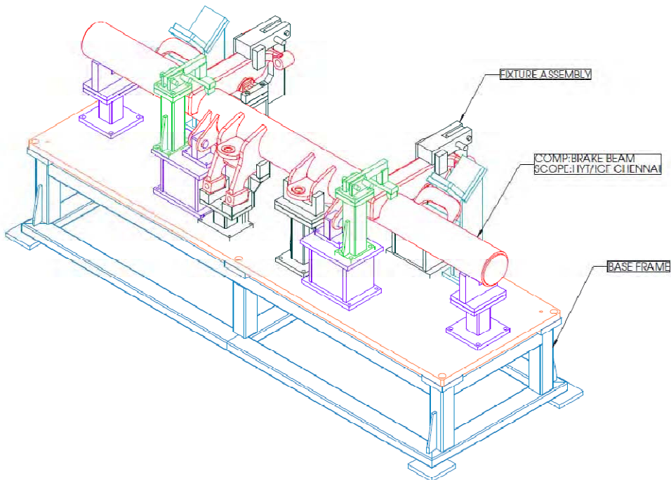
Brake Beam Tack Weld Fixture
